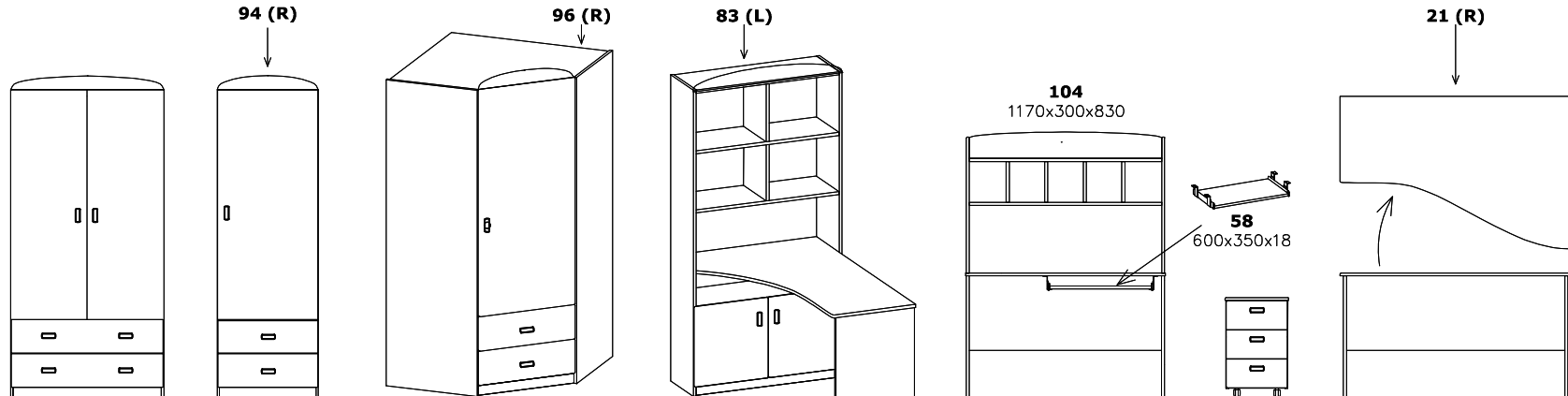
93 895x566x1800(+100) 94 (R) 595x566x1800(+100) 95 (L) 96 (R) 985x985x1800(+100) 97 (L) 83 (L) 895(510)x1320x1800(+100) 82 (R) 104 1170x300x830 47 1200x540x730 58 600x350x18 46 380x450x600 21 (R) 1300x900(510)x730 22 (L)
