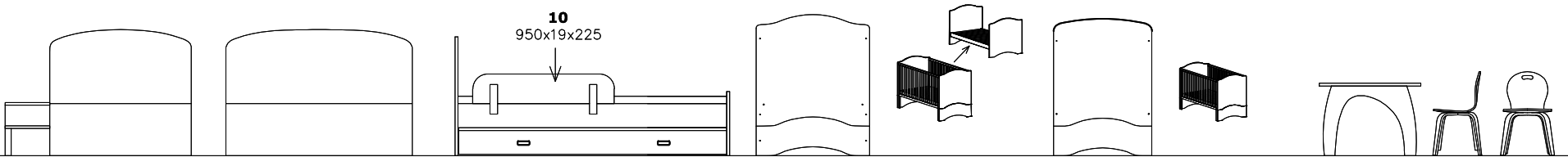
90 1940x950x850(350) 91 1940x1250x850(350) 10 950x19x225 92 1890x855x140 14 1422x760x940 70 1222x660x920 23 670x670x500 103 300x340x565 13 350x350x335
